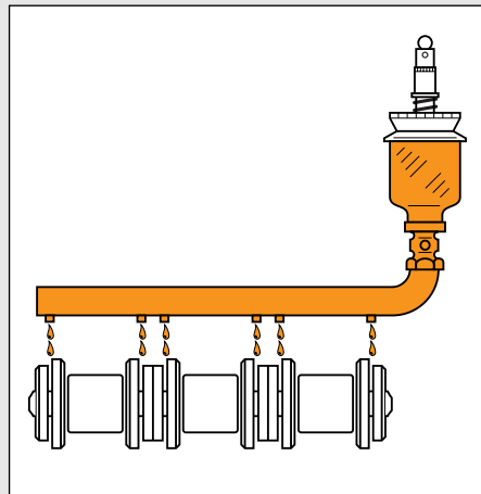
Fig. 6: Drip lubrication.
