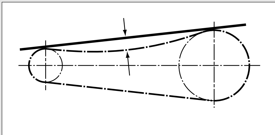
Fig. 8: Chain tension – slack determination.
